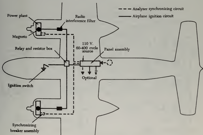
FIGURE 4-72. Twin-engine analyzer installation.
